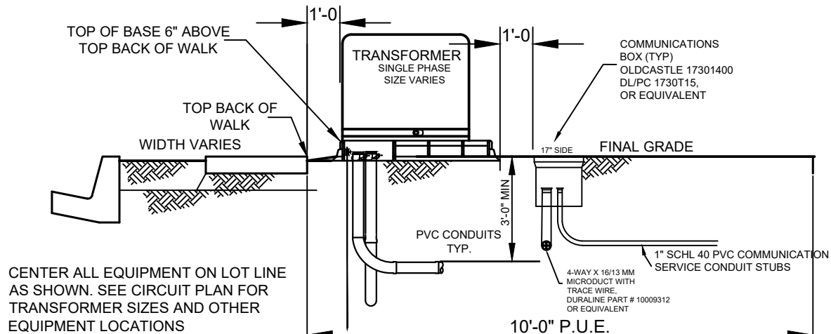
( SECTION VIEW )
