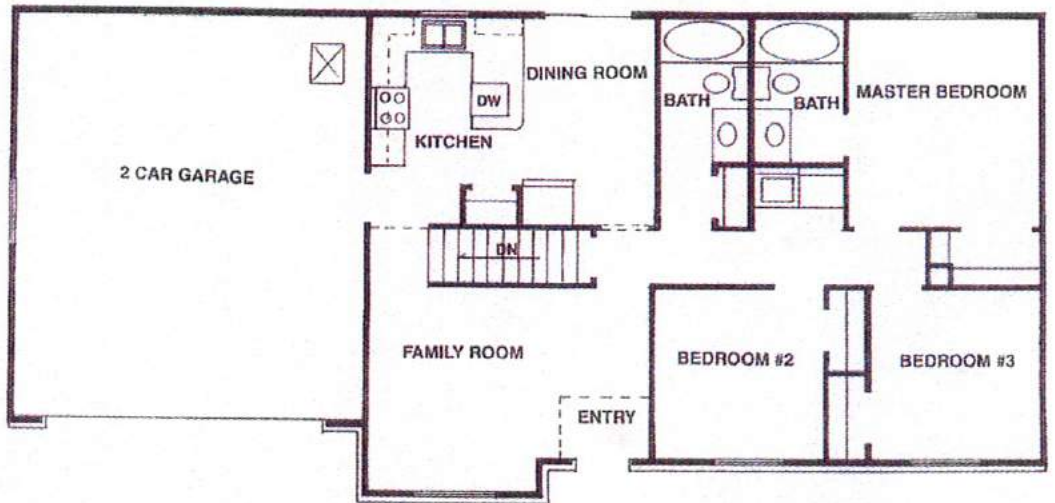
MAIN FLOOR
