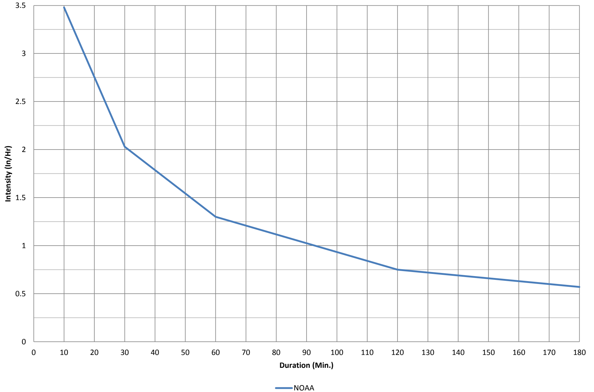
Intensity Duration Curve - 100 Yr.
