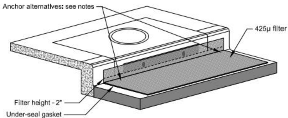
ERTEC® Combo Guard™ Protected drainage Inlet
