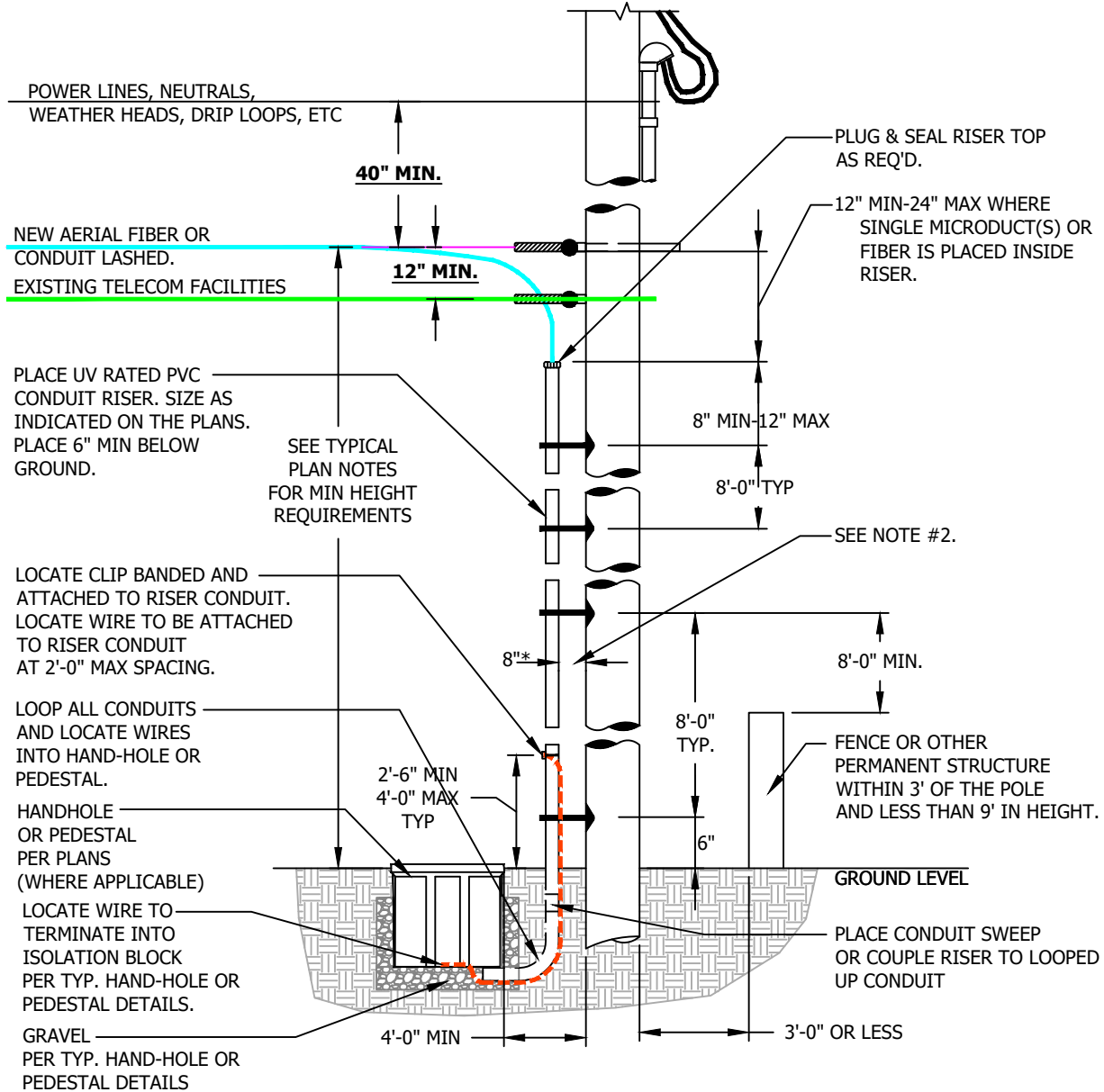
TYPICAL RISER DETAIL ON SHARED POLE
