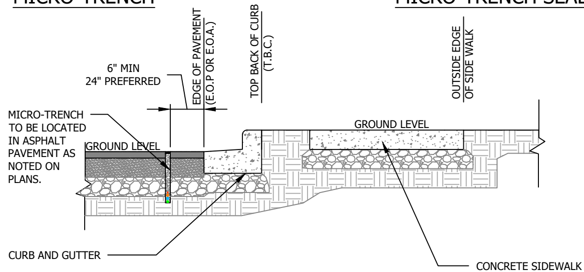
TYPICAL MICRO-TRENCH DETAIL
