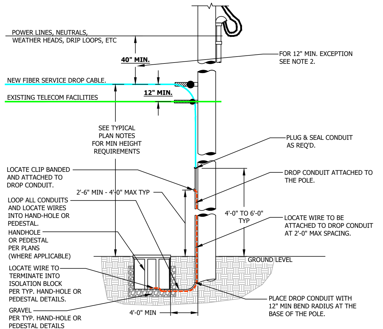
TYPICAL DROP CONDUIT POLE ATTACHMENT
