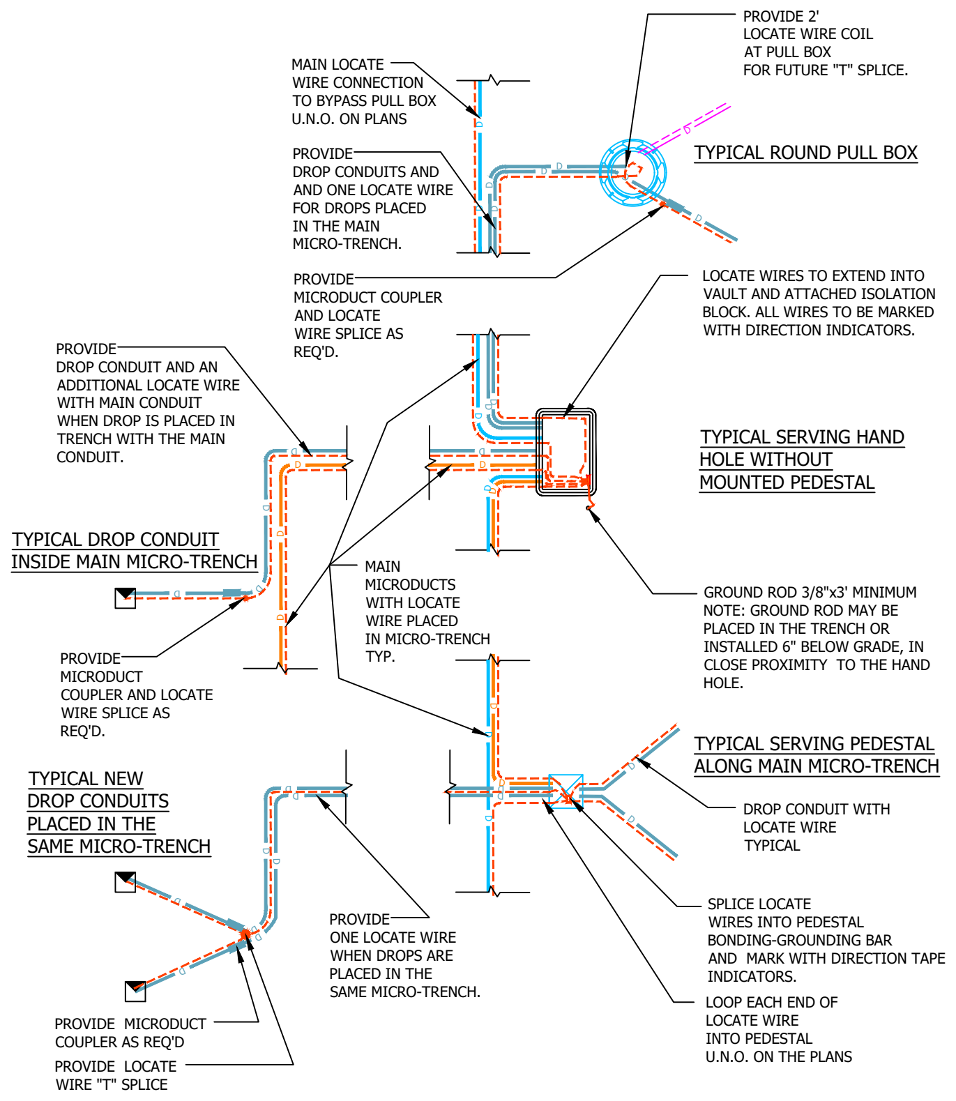
MICRO-TRENCH LOCATE WIRE DETAIL
