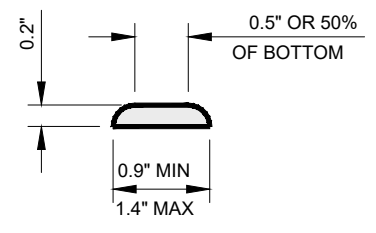
DETECTABLE RAMP DETAIL
