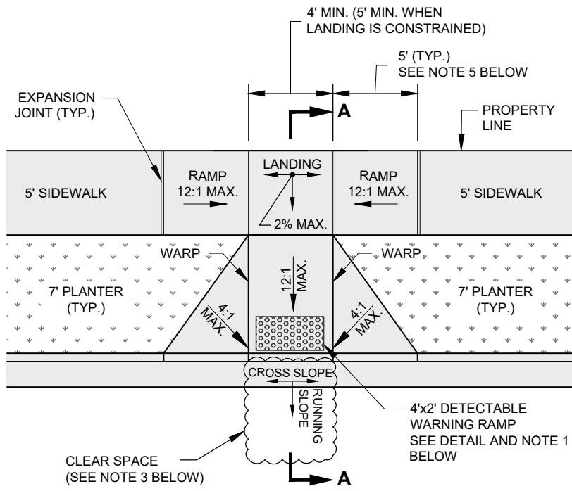
PLAN VIEW
